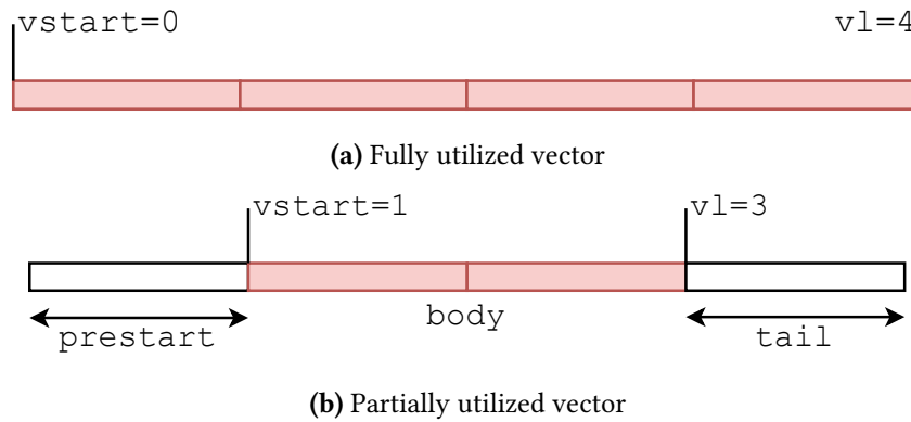
Figure 2.4: Examples of vector utilization with v1 and vstart
