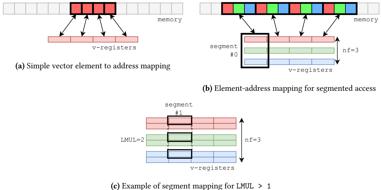
Figure 2.8: Comparison between segmented and unsegmented accesses For readability, the vector registers are 2x as wide
